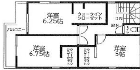
2F:52.17㎡
